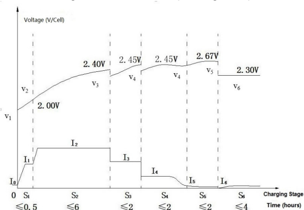
Charge Curve for 6-EVF-80(for Single Cell)
